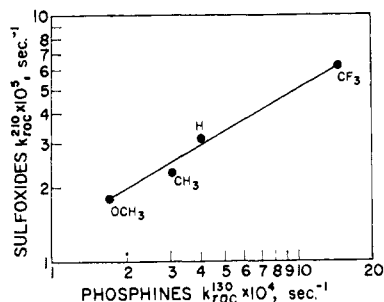
Figure 1. Correlation of \log k_{\text{rac}} values of arylmethylphenylphosphines and aryl p -tolyl sulfoxides (aryl = p -RC 6 H 4 ). See ref 35.
